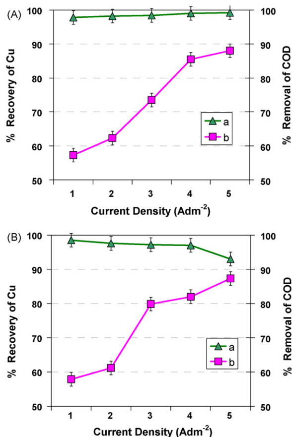
Fig. 3. Effects of current density on the efficiency of (a) recovery of Cu and (b) COD removal in the electrochemical treatment of Cu-phthalocyanine dye process stream at different temperatures after a 5-h electrolysis. Experimental conditions: (A) T = 30 °C and (B) T = 50 °C, anode: DSA.
