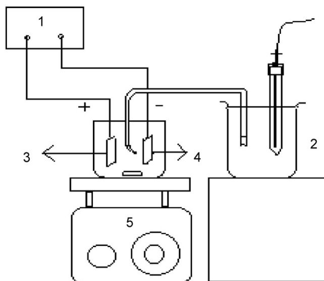
Fig. 1. A schematic view of batch experimental setup: 1. power supply 2. reference electrode 3. anode 4. cathode 5. magnetic stirrer.
