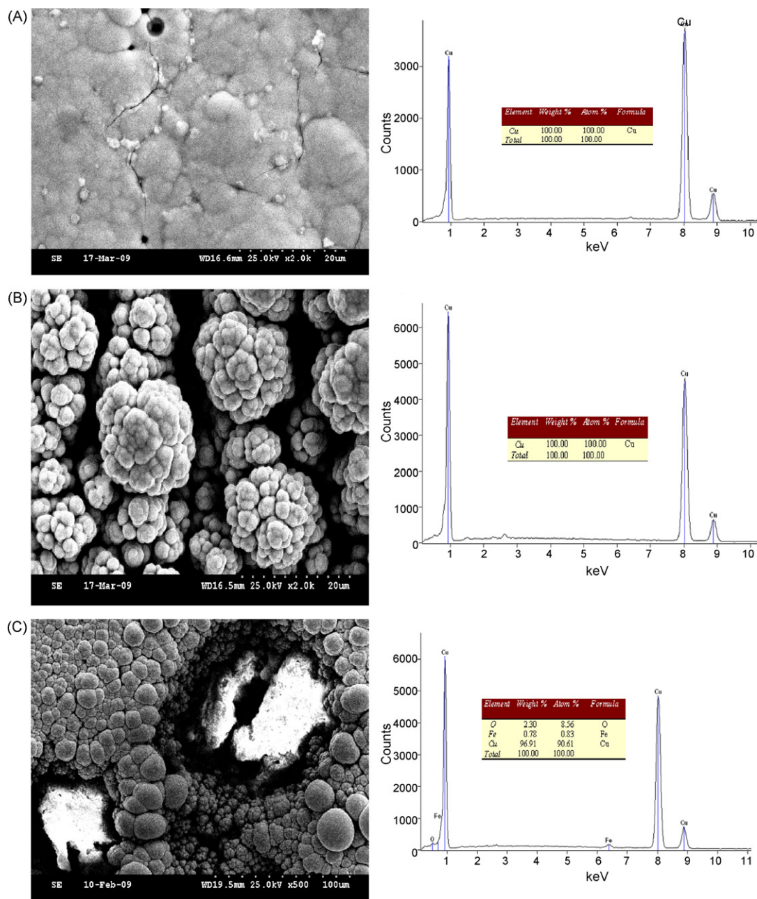
Fig. 4. SEM surface images and EDX spectrum of copper deposition on stainless steel plate from the copper-phthalocyanine process stream at different current densities: (A) 1 A dm -2 (100% Cu), (B) 5 A dm -2 (100% Cu), and (C) 5 A dm -2 . Oxide formation (96.9% Cu).
