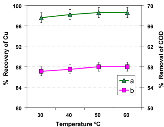
Fig. 2. Effects of temperature on the efficiency of (a) recovery of Cu and (b) COD removal in the electrochemical treatment of Cu-phthalocyanine dye process stream after a 5-h electrolysis. Experimental conditions: CD: 1 A dm -2 , anode: DSA.
