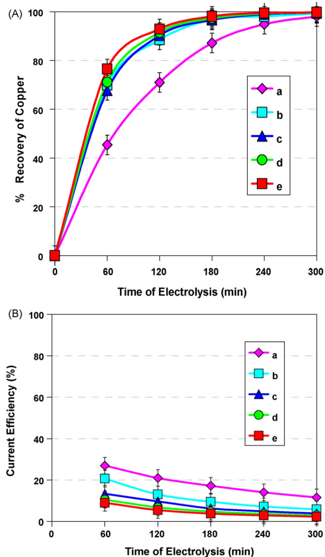
Fig. 5. Effects of cathodic current density on copper recovery from the Cu-phthalocyanine dye process stream during the electrolytic treatment. (A) Copper recovery efficiency and (B) current efficiency. Experimental conditions: CD (A dm -2 ) (a) 1, (b) 2, (c) 3, (d) 4, and (e) 5. T = 30 °C, anode: DSA.
