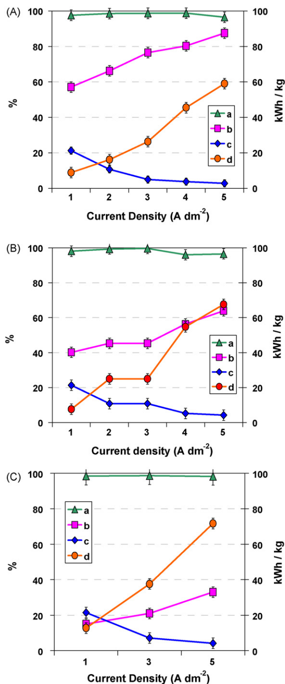
Fig. 6. Effect of current density on the electrochemical treatment of Cu-phthalocyanine dye process stream using different anode materials after a 5-h of electrolysis. (A) RuO 2 /Ti, (B) SnO 2 /Ti, and (C) Graphite. (a) Recovery of Cu (%), (b) COD removal (%), (c) cathodic current efficiency (%), and (d) energy consumption for removal of copper (kWh/kg). Experimental conditions: T = 30 °C.
